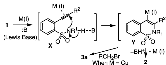
SCHEME 3. Proposed Mechanism for the Formation of Benzothiazines
